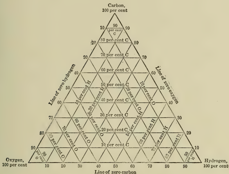
FIG. 11.—Trilinear Coordinates on an Equilateral Triangle.
